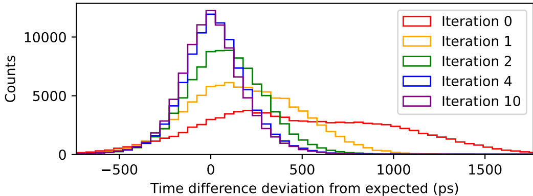
Time difference deviation from expected, channel 2439
